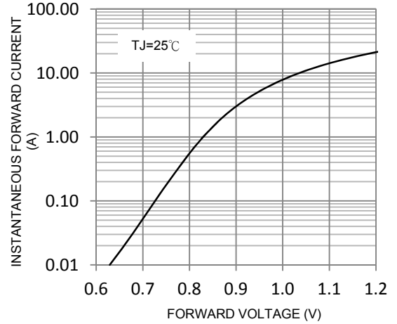
FIG. 2-Typical Forward Characteristics
