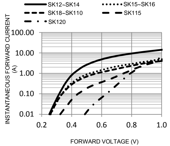
FIG. 2-Typical Forward Characteristics
