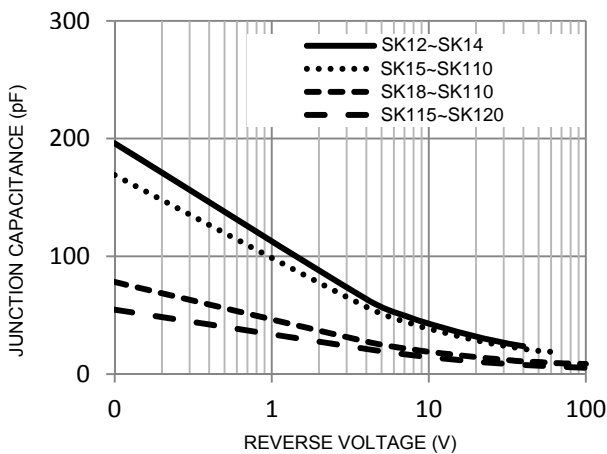
FIG. 5-Typical Junction Capacitance
